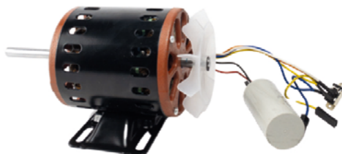
Motor 4P 1/3 127-220V REF: 3100055
